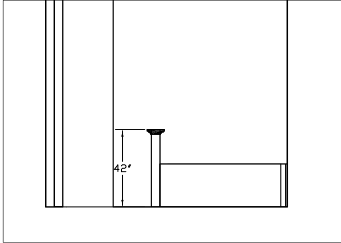
1 BATHROOM WALL A1.3
